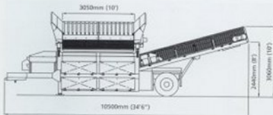
Powertrack 800 in Working Position.
