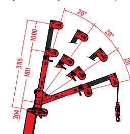
Fly Jib - 800kg Maximum Capacity
