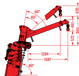
Fly Jib - 800kg Maximum Capacity
