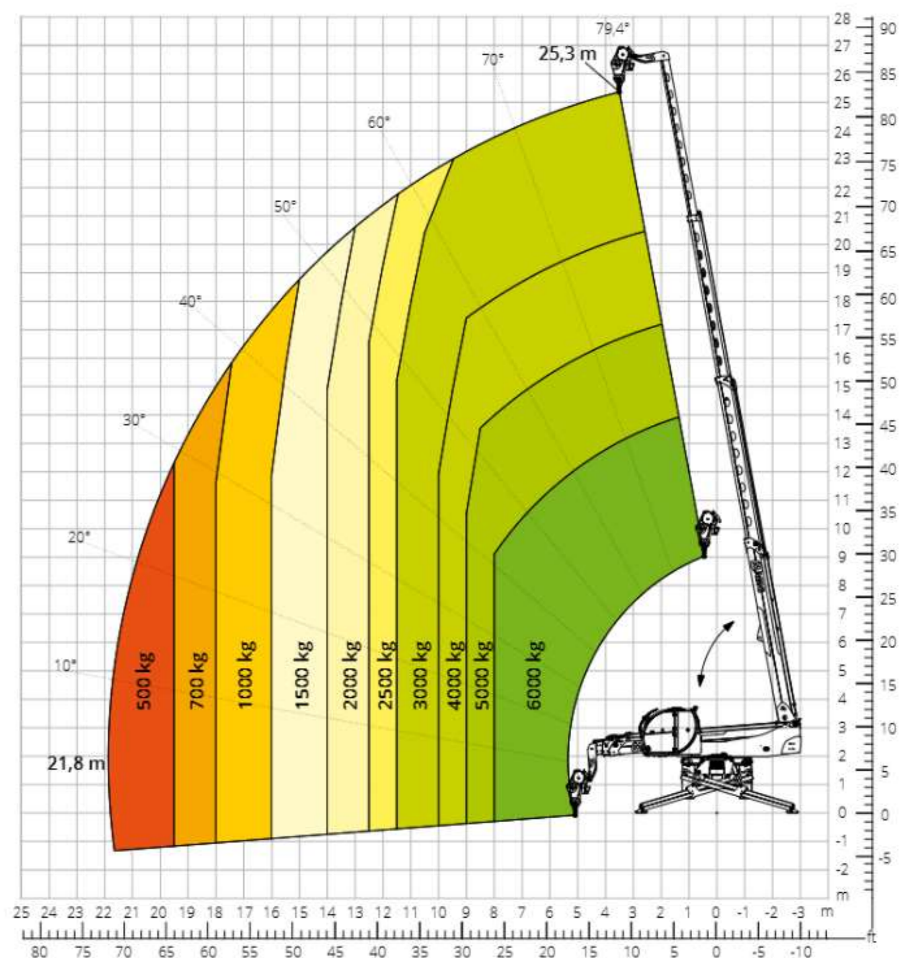
Load chart with WINCH, 6,000 kg ATT - 02 - 004
