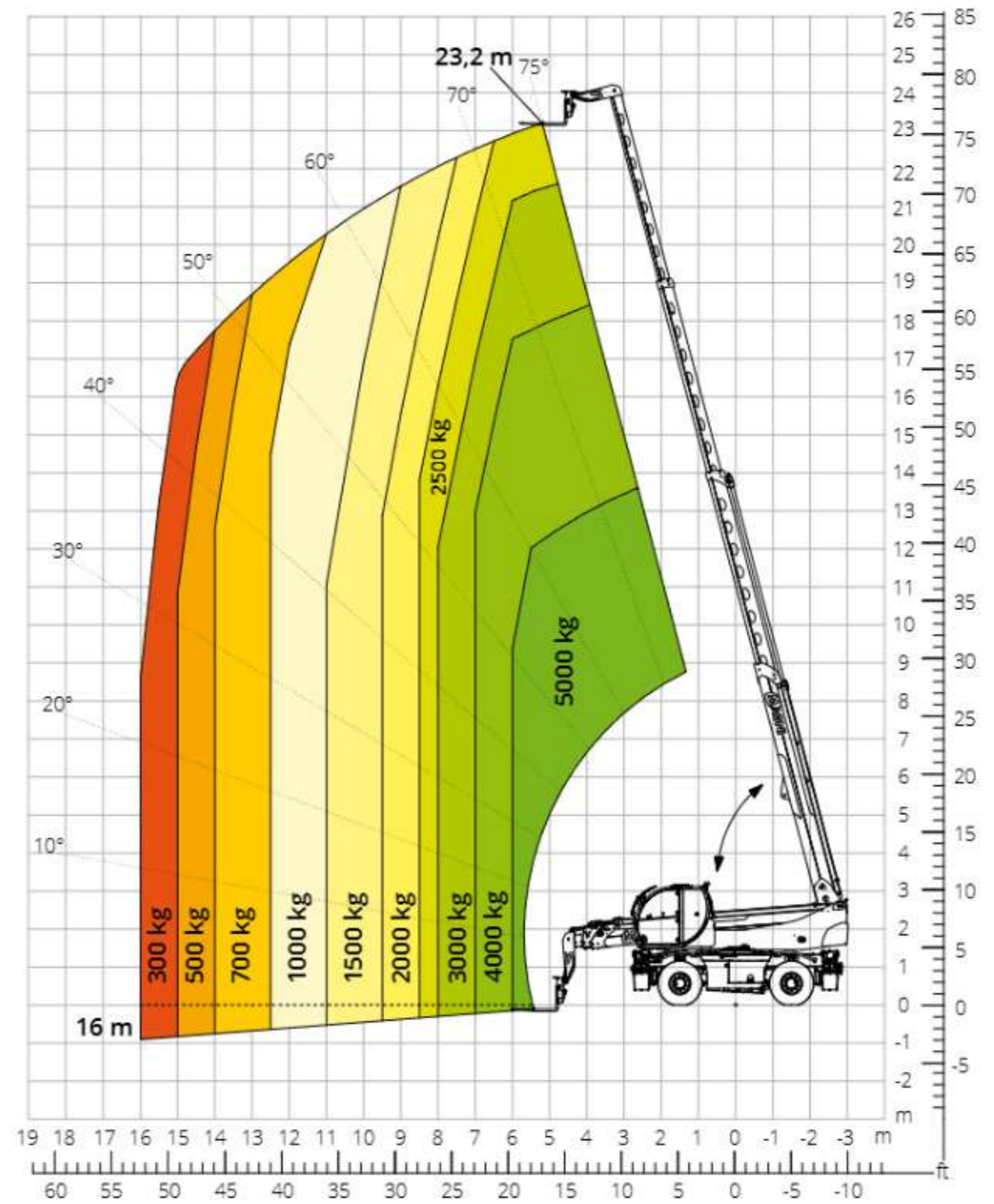
Load chart FRONT ATTACHMENT ON TYRES ATT-03-004
