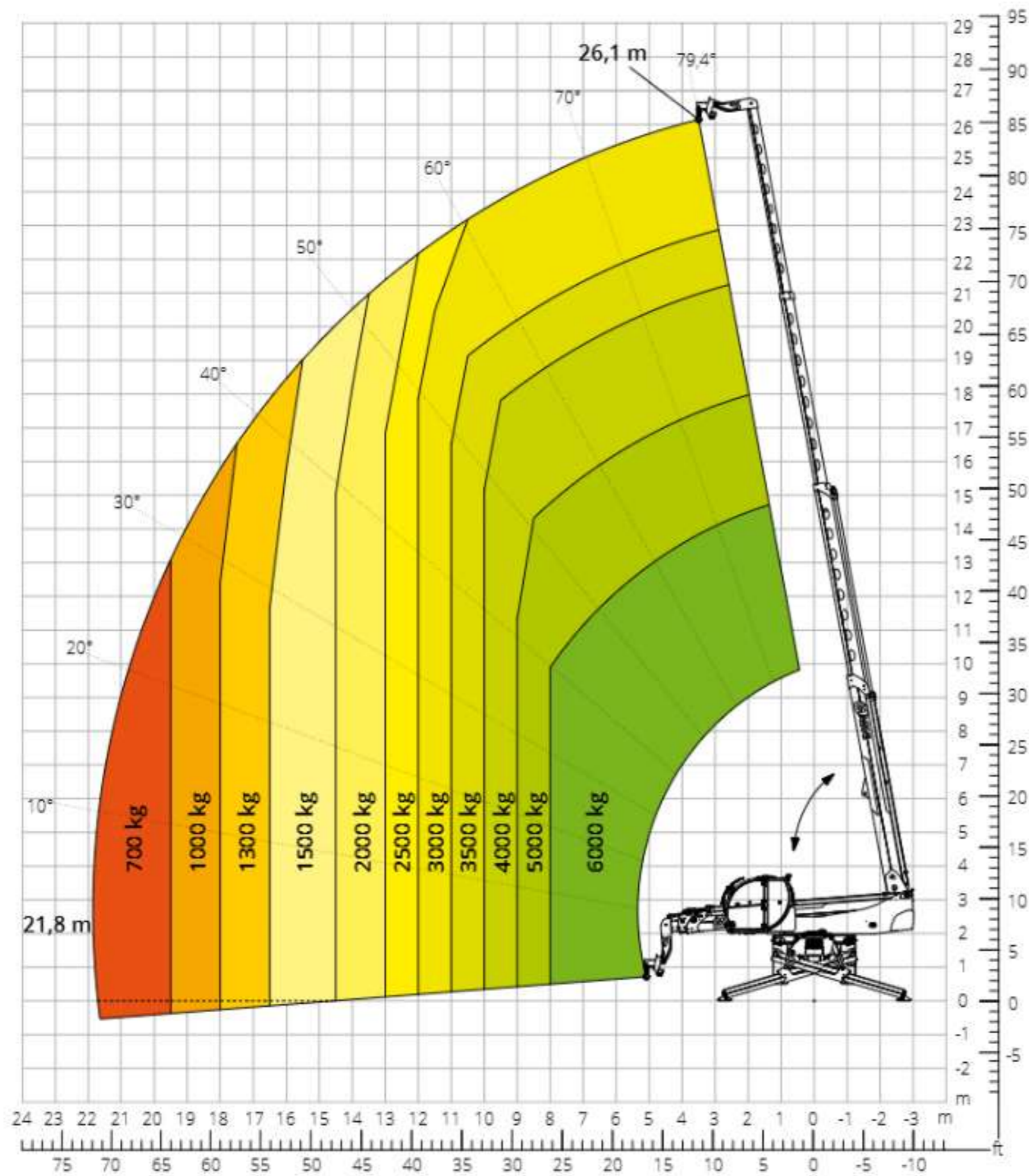
Load chart with HOOK, 6,000 kg ATT - 05 - 001
