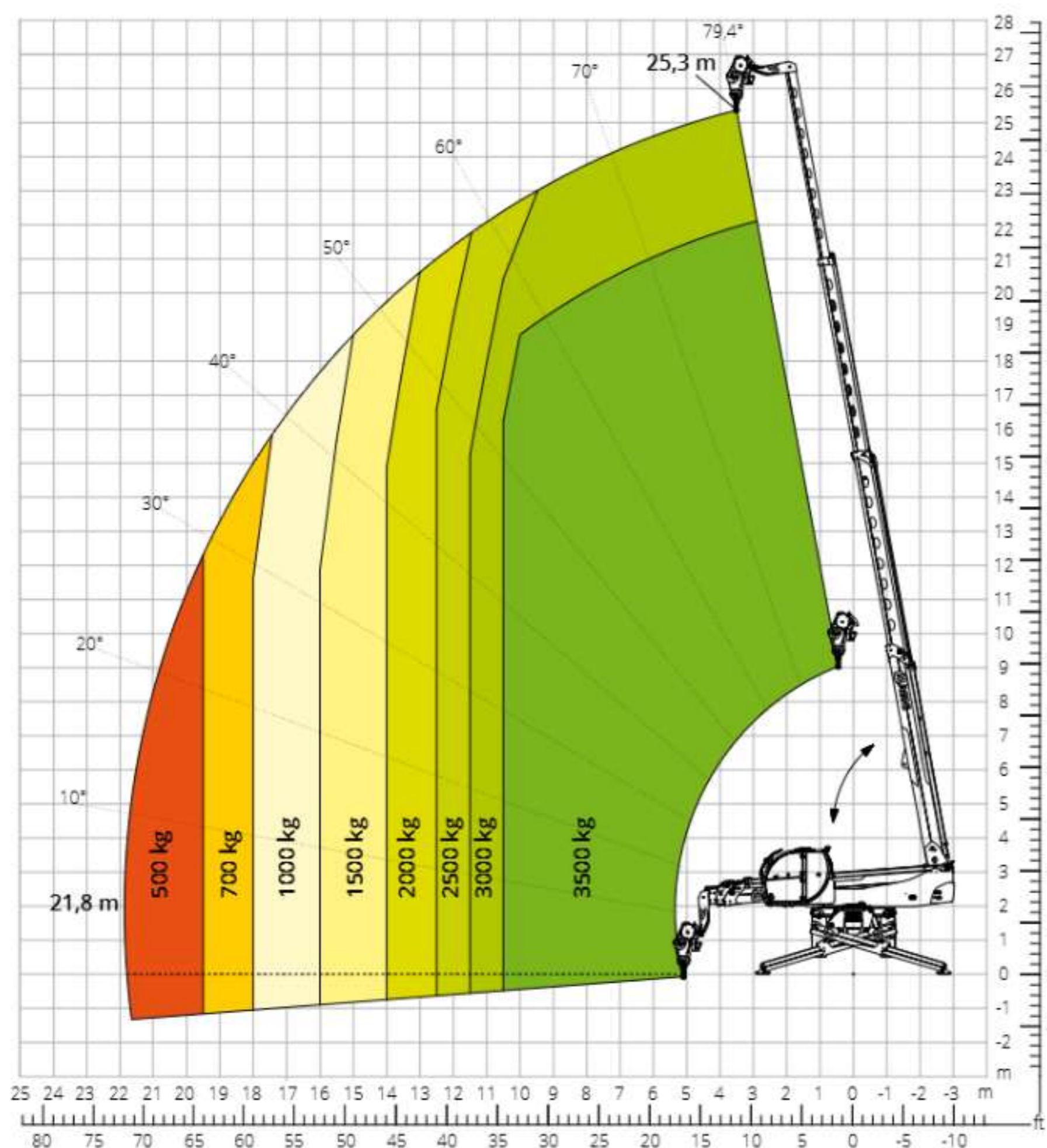
Load chart with WINCH, 3,500 kg ATT - 02 - 002
