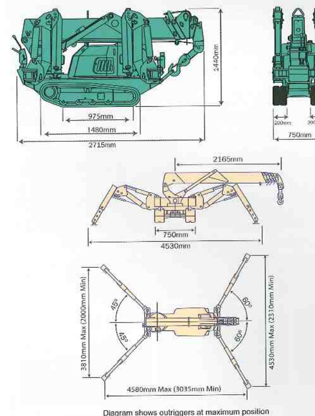
Diagram shows outriggers at maximum position
