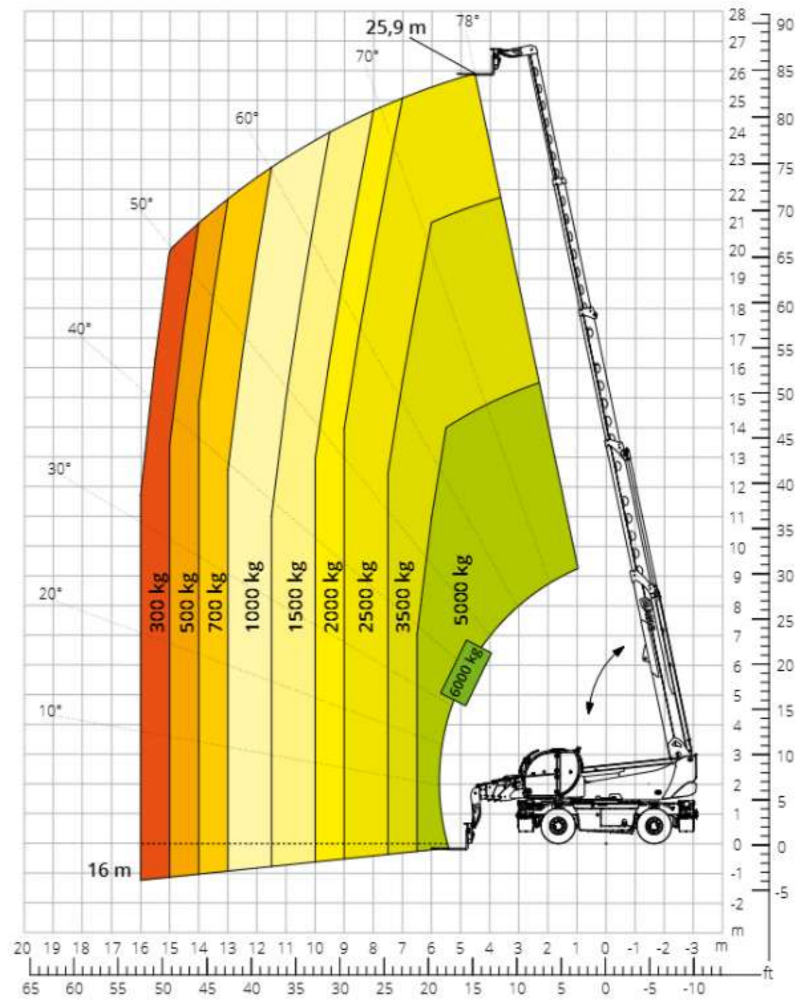
Load chart FRONT ATTACHMENT ON TYRES ATT-03-004
