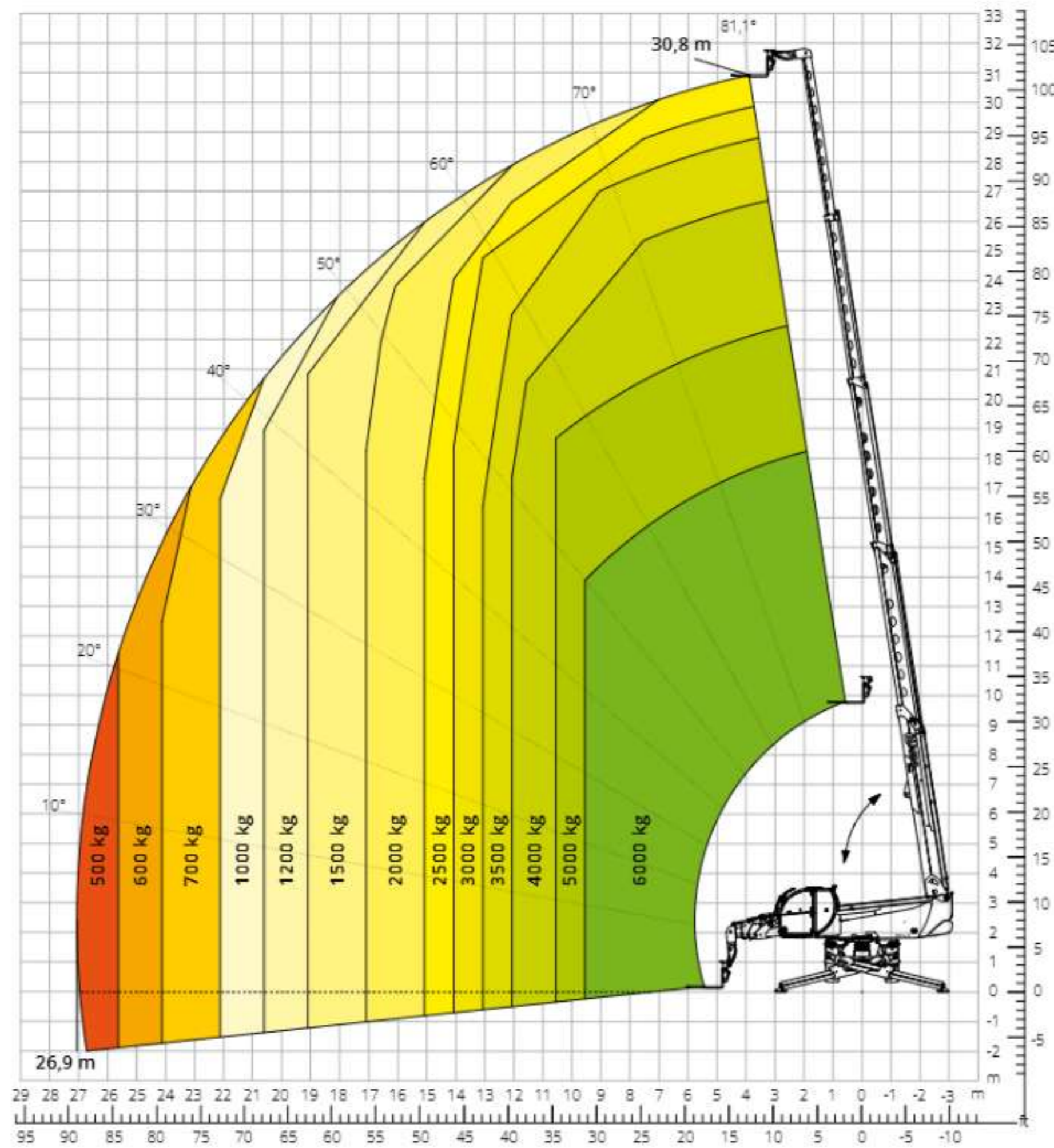
Load chart with FULLY EXTENDED STABILISERS (360°) ATT-03-004
