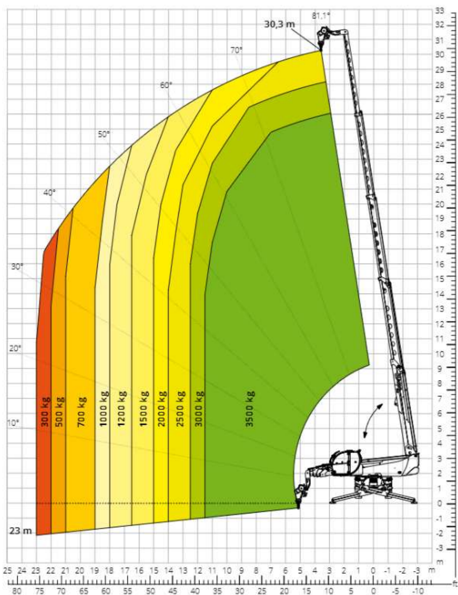
Load chart with WINCH, 3,500 kg ATT - 02 - 002
