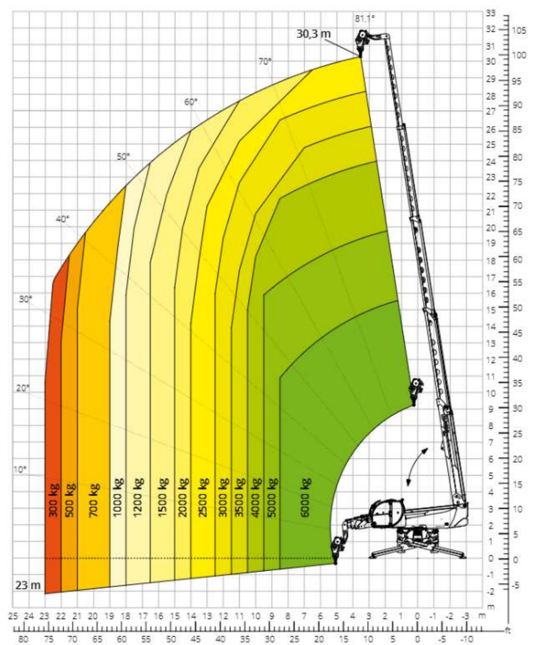
Load chart with WINCH, 6,000 kg ATT - 02 - 004
