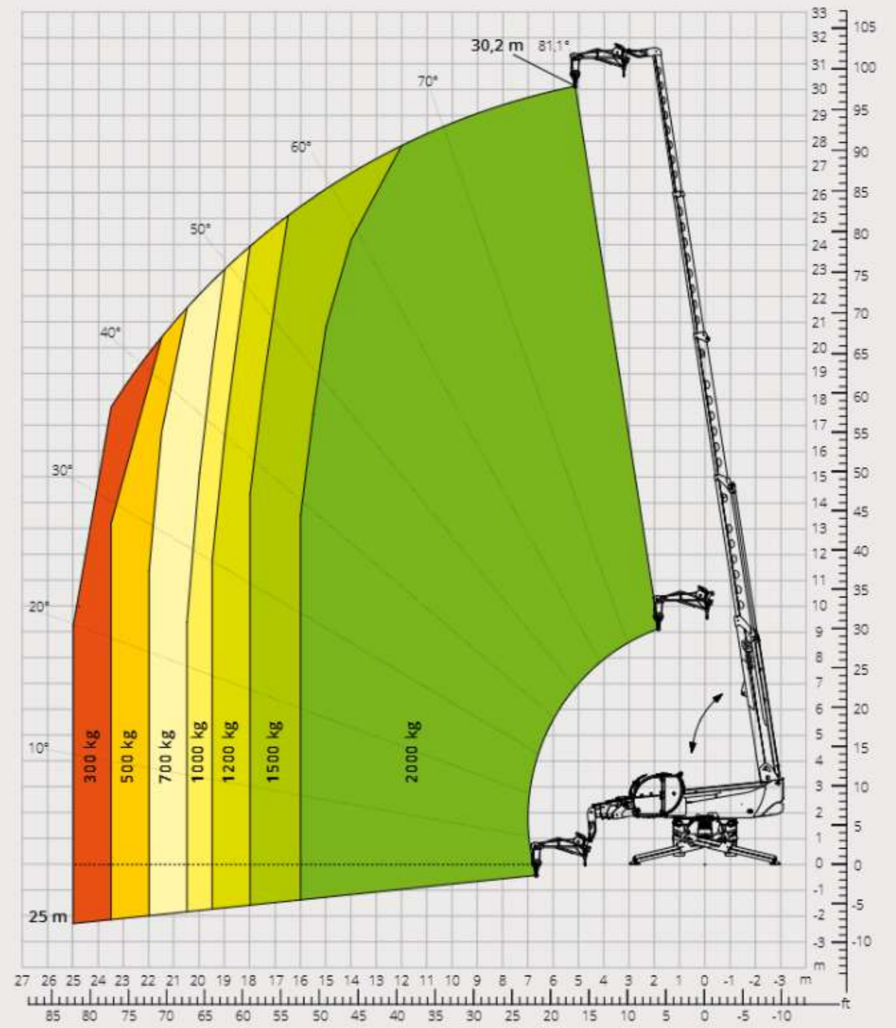
Load chart with JIB WITH WINCH, 2,000 kg ATT - 04 - 015
