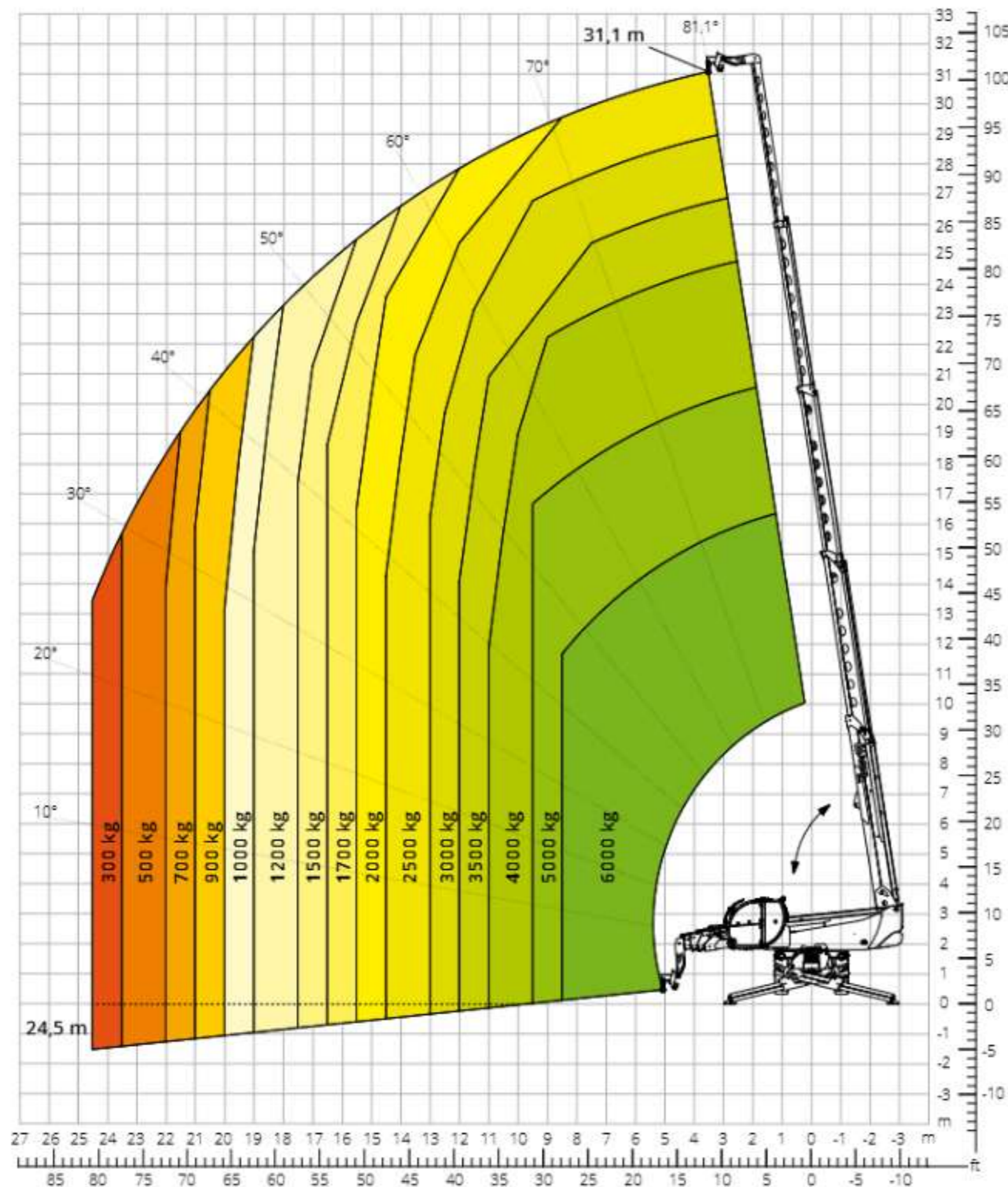
Load chart with HOOK, 6,000 kg ATT - 05 - 001
