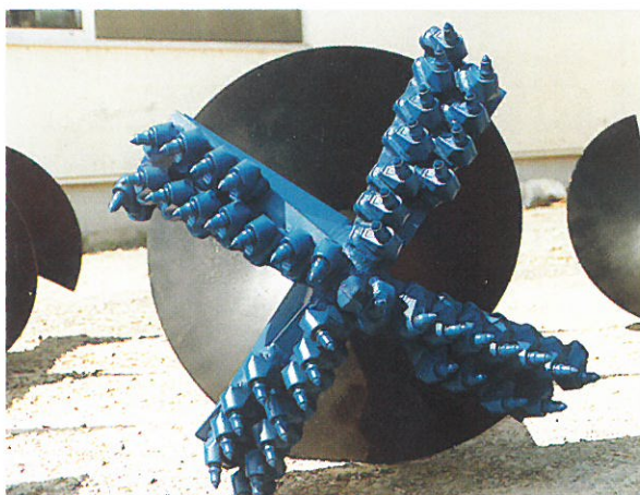
Horizontal-Bohrkopf DN-R
