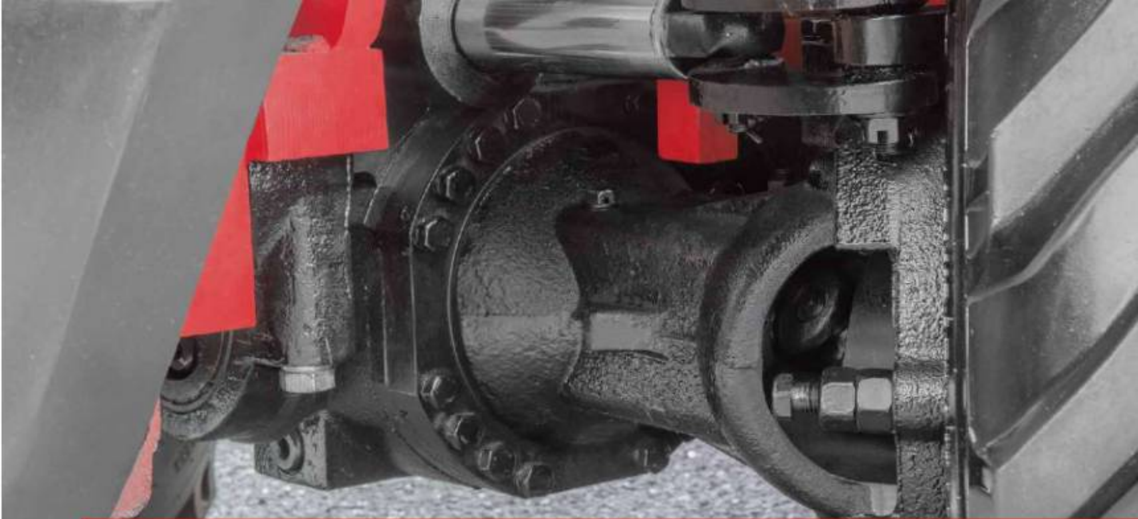
Oscillating steer axle allows either wheel to step over obstacles keeping the truck and load level.
