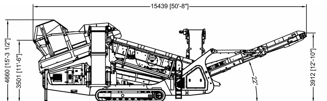
3-WAY SPLIT WORKING ARRANGEMENT HOPPER EXTENSIONS FITTED
