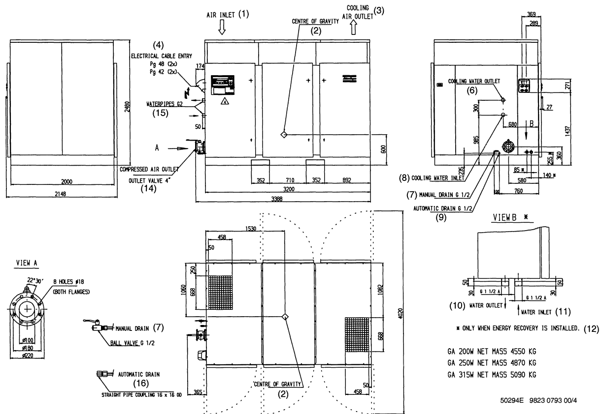
Fig. 6f. Dimension drawing GA W 200 up to -315
