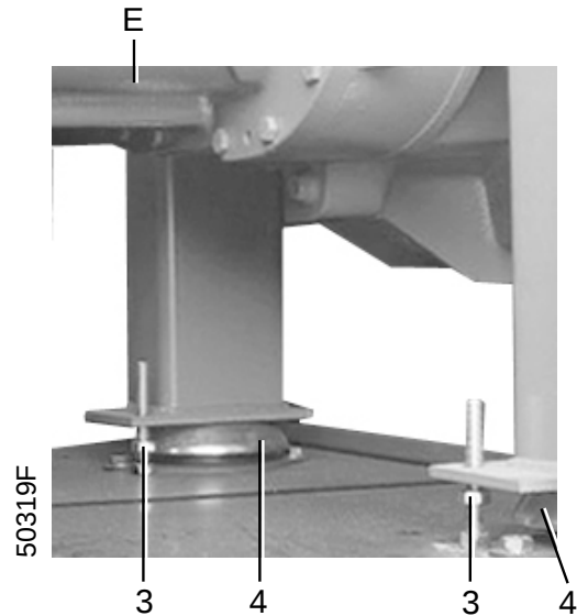
Fig. 11a Gear casing side
