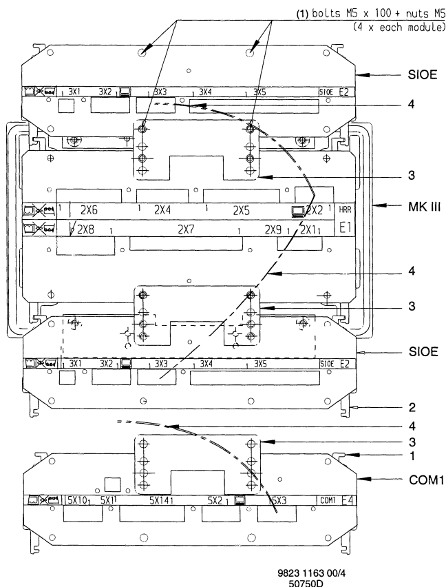
Fig. 4. Installation of communication module (typical example)
