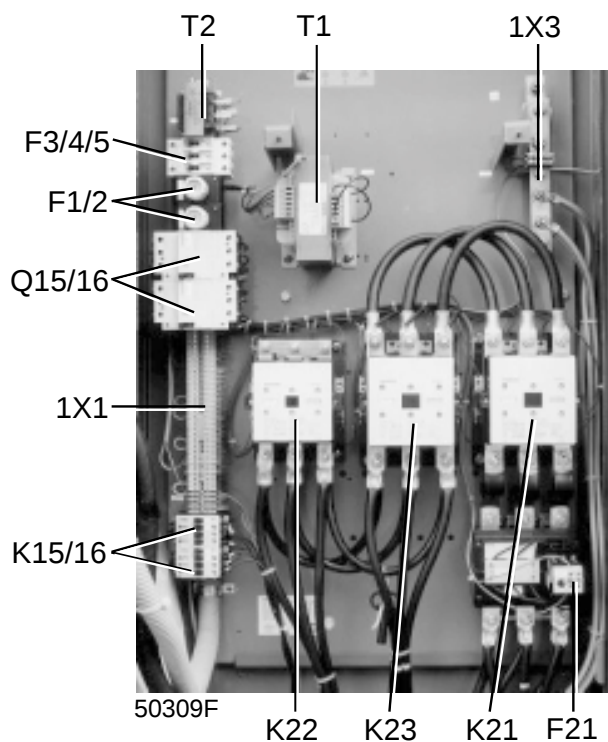
Fig. 2. Electric cabinet (typical example)
