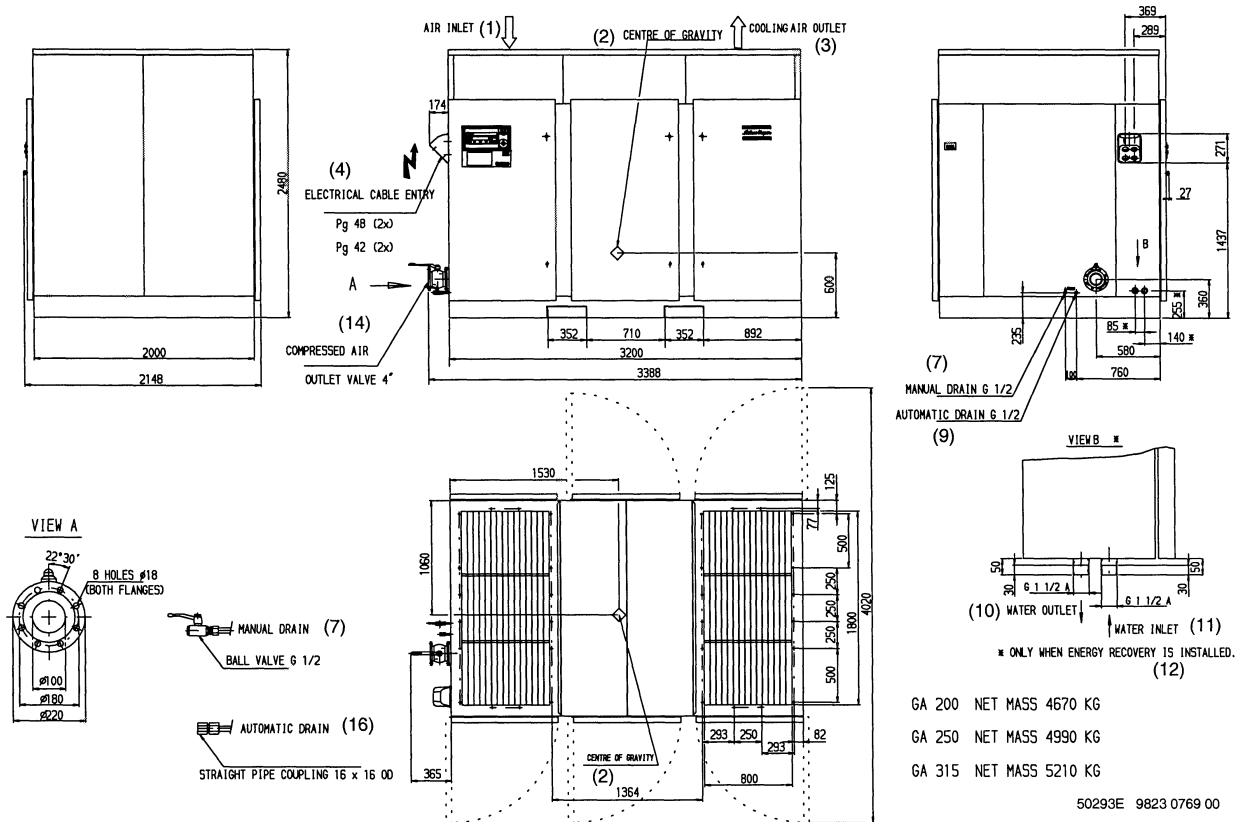
Fig. 6e. Dimension drawing GA200 up to -315
