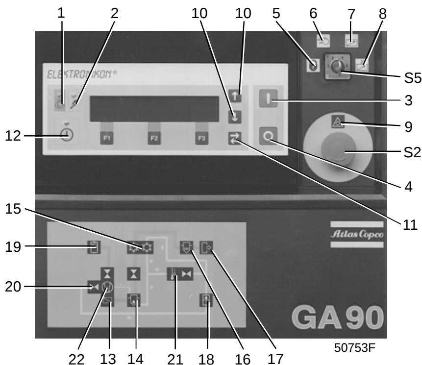
Fig. 10a. Pictographs on control panel
