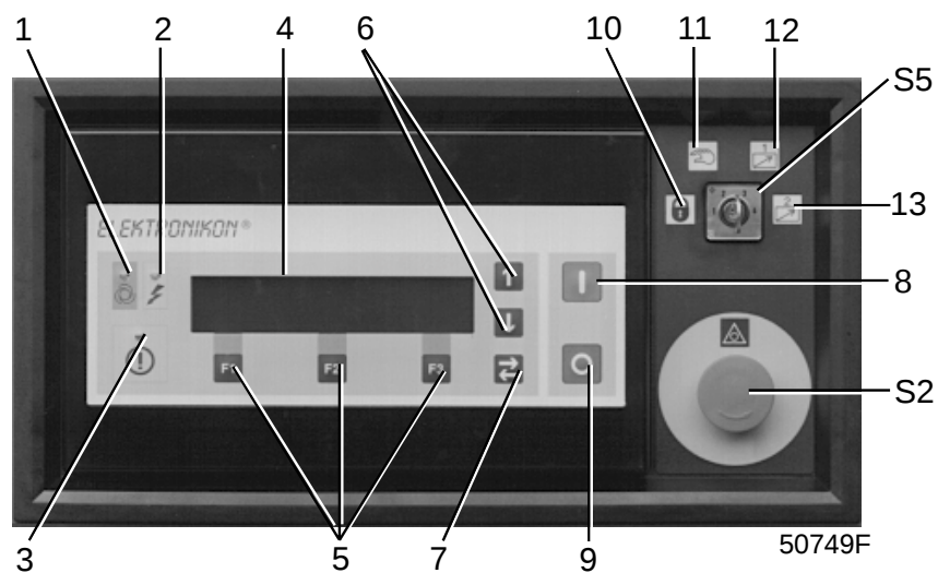
Fig. 3a. Control panel
